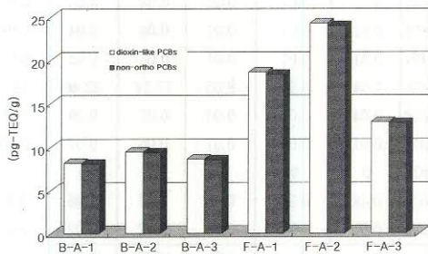
Fig. 2. The level of dioxin-like PCBs and non-ortho PCBs
