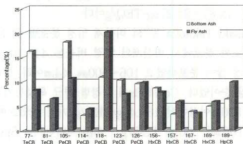
Fig. 3. Distributions of PCBs(pg/g %, dry weight)
