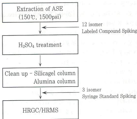
Fig. 1. A flow chart of dioxin-like PCBs
